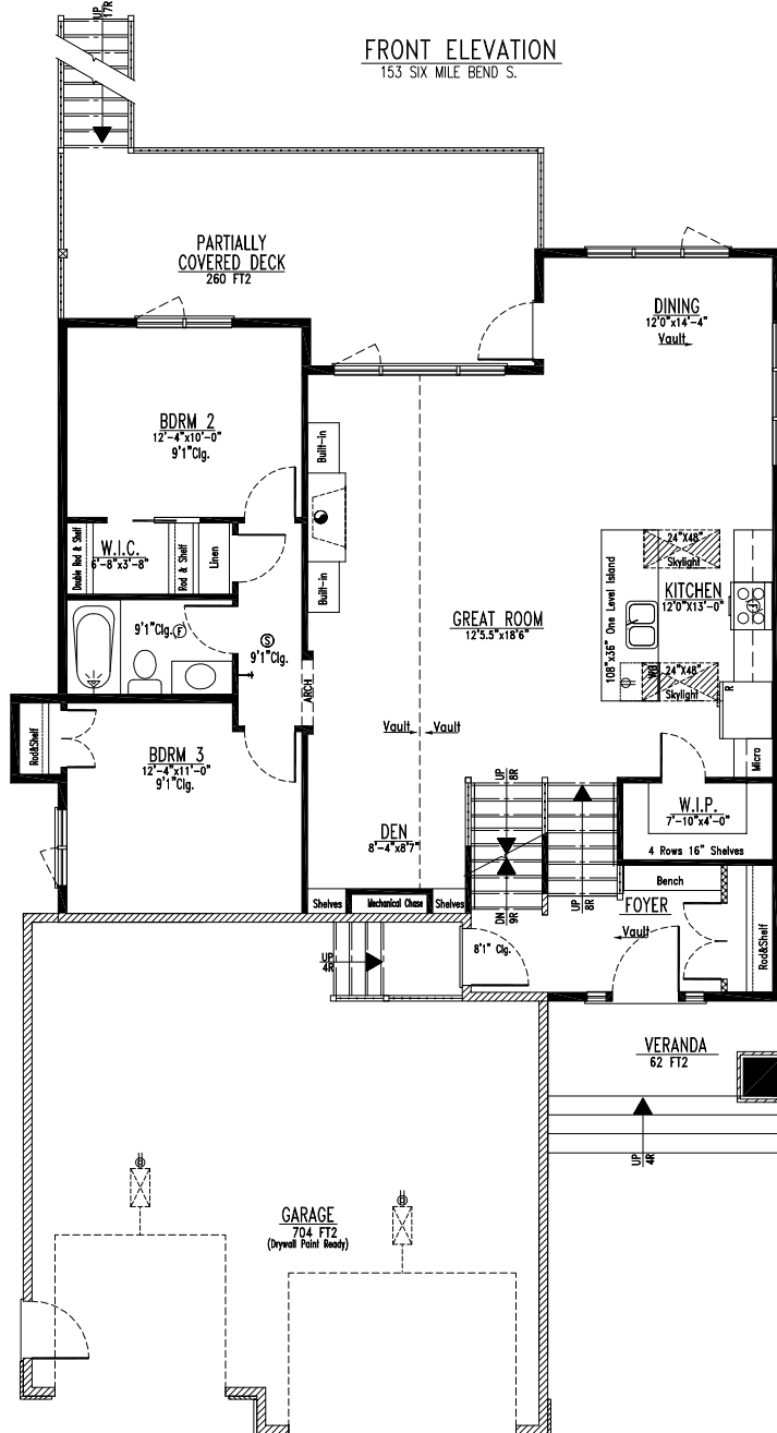
MAIN LEVEL FLOOR PLAN 1,315 FT 2 153 SIX MILE BEND S. OCT.14, 2015
