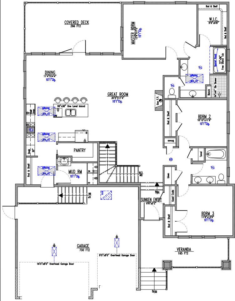
MAIN LEVEL FLOOR PLAN 2,010 FT 2 24 STONECREST POINT W. SEPT. 24, 2014
