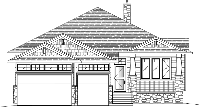
FRONT ELEVATION 24 STONECREST POINT W.
