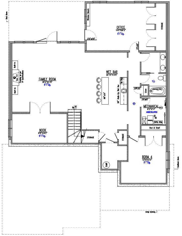
LOWER LEVEL DEVELOPMENT 1,870 FT 2
