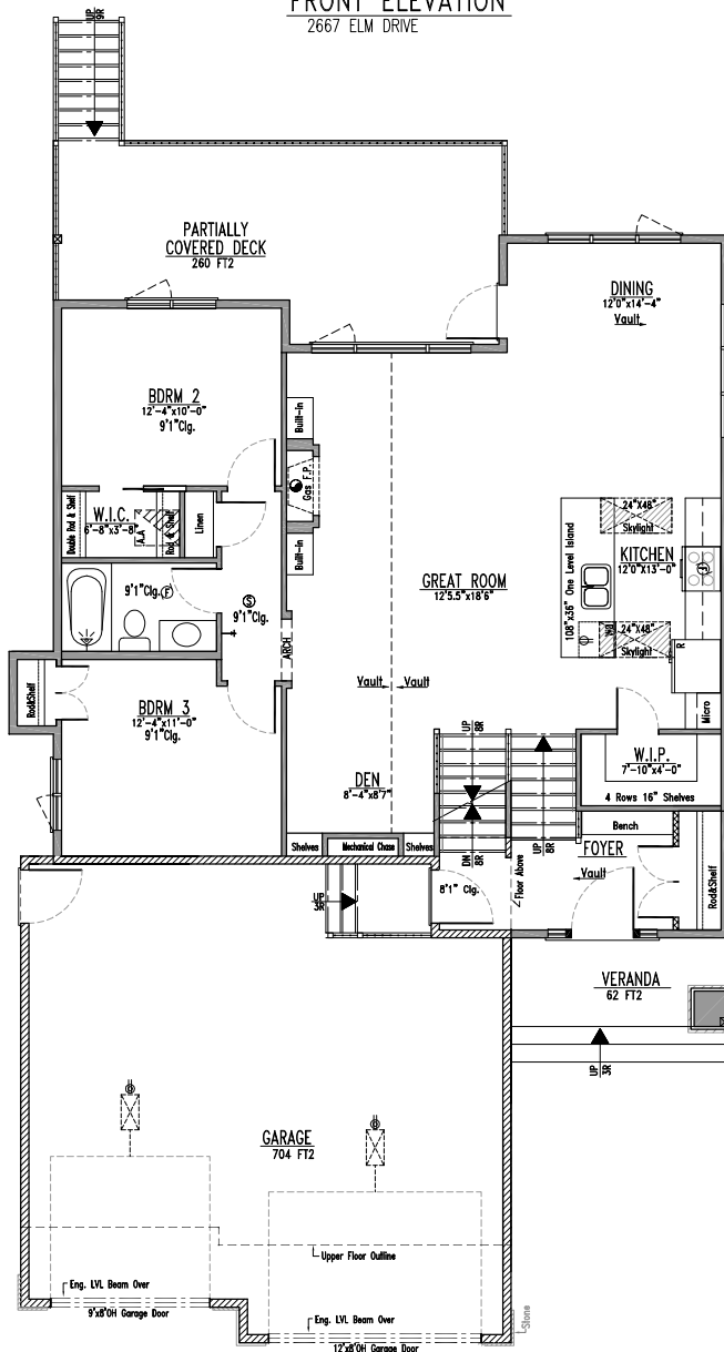
MAIN LEVEL FLOOR PLAN 1,315 FT2 2667 ELM DRIVE MAR.03/15
